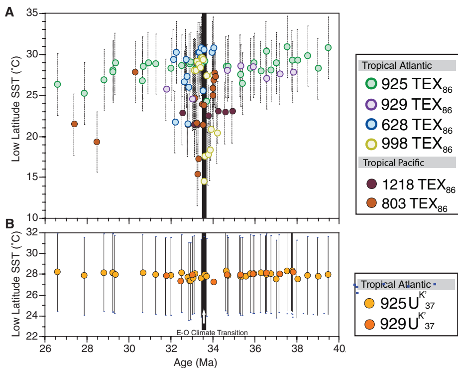
Fig. 3. Tropical SST records during the late E-O. (A) \text{TEX}_{86} SST records from six tropical sites. (B) U^{K'}_{37} -SST records from sites 925 and 929. The \text{TEX}_{86} proxy probably overestimates the magnitude of tropical SST changes because of tropical oceanographic perturbations associated with high-latitude cooling.
