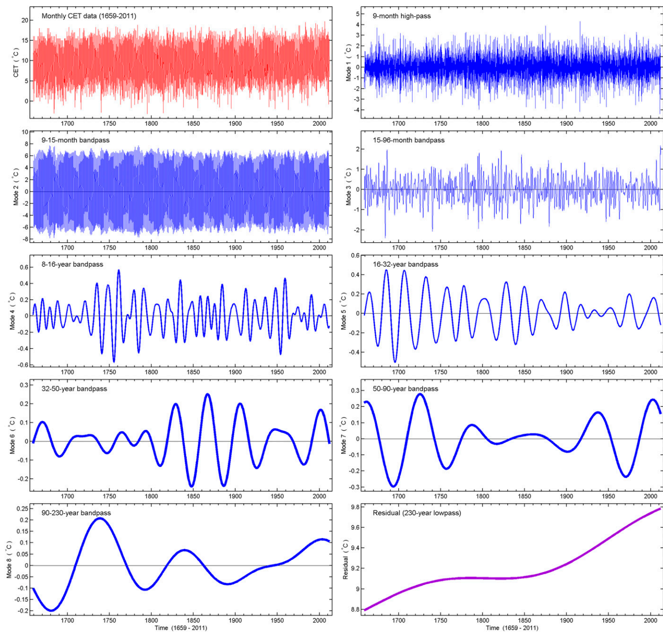
Fig. S2. Wavelet reconstruction of the original time Central England Temperature series is shown in the first panel. The other panels are various band-filtered parts that together reconstruct the original data.
