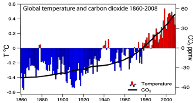
Fig. 1. Time series of annual global mean temperature departures for 1861-2008 from a 1961-90 mean (bars), left scale, and the annual mean carbon dioxide from Mauna Loa after 1957 linked to values from bubbles of air in ice cores prior to then. The zero value for 1961-90 for temperature corresponds to 14°C and for carbon dioxide 334 parts per million by volume (ppmv). Updated from Karl and Trenberth 16 ; original data from HADCRUV3 http://www.cru.uea.ac.uk/cru/data/temperature/#datadw , and http://www.esrl.noaa.gov/gmd/ccgg/trends/ .
