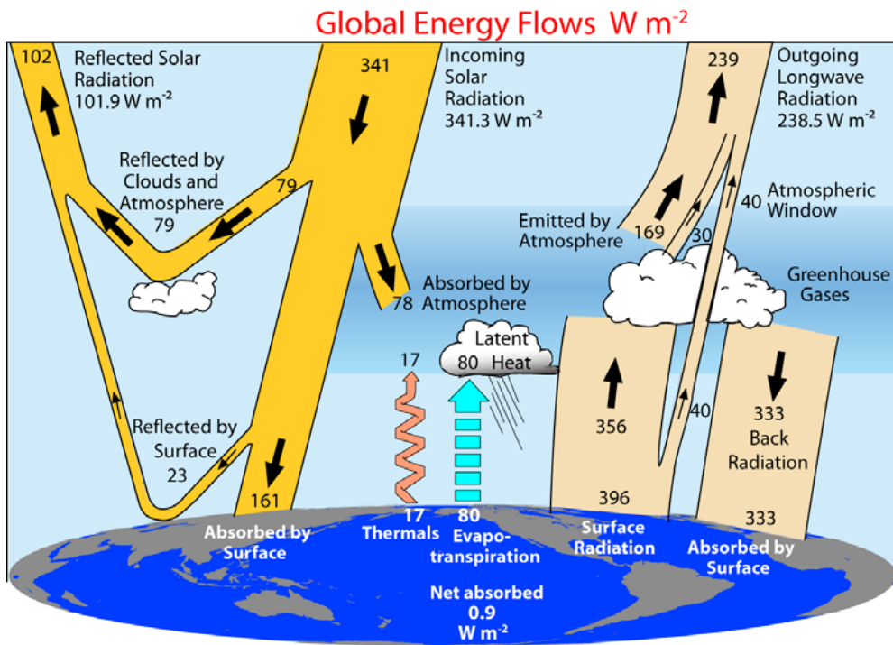
Fig. 2. The global annual mean Earth's energy budget for the March 2000 to May 2004 period in W m^{-2} . The broad arrows indicate the schematic flow of energy in proportion to their importance. From Trenberth et al. 6
