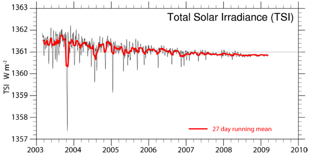
Fig. 5. Daily total solar irradiance from the Total Irradiance Monitor (TIM) instrument on the Solar Radiation and Climate Experiment (SORCE), along with a 27-day running mean in red. http://lasp.colorado.edu/sorce/index.htm (Data courtesy Laboratory for Atmospheric and Space Physics, U Colorado.)
