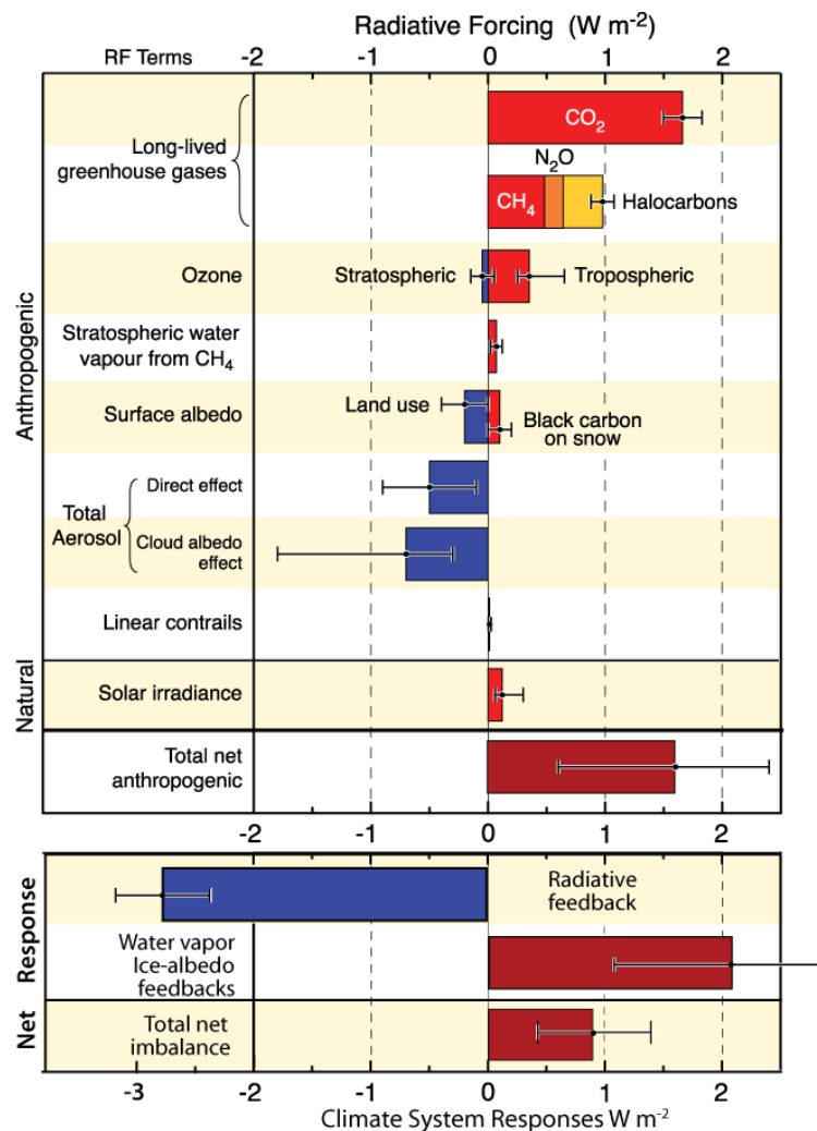
Fig. 4. The top part of the figure is the radiative forcing from IPCC 1 with the agents of change in left column and radiative forcing \text{W m}^{-2} with 90% confidence limits. The lower part shows estimates of the main negative radiative feedback, the water vapor, ice-albedo and other feedbacks, and the net radiative imbalance. Error bars for the latter are based on Fasullo and Trenberth 7 and others are approximate.
