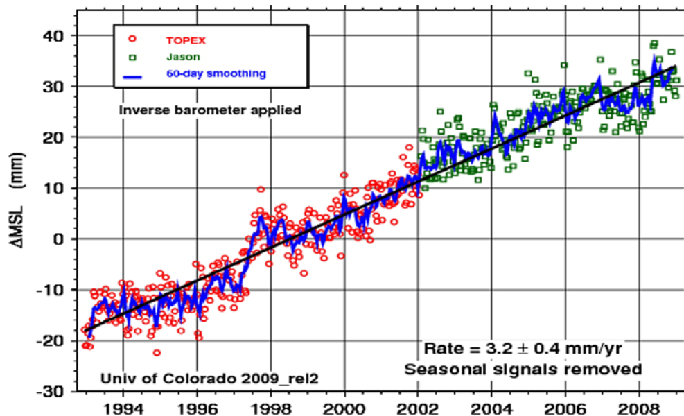
Fig. 3. Global sea level since August 1992. The TOPEX/Poseidon satellite mission provided observations of sea level change from 1992 until 2005. Jason-1, launched in late 2001 continues this record by providing an estimate of global mean sea level every 10 days with an uncertainty of 3-4 mm. The seasonal cycle has been removed and an atmospheric pressure correction has been applied. http://sealevel.colorado.edu/ . Courtesy Steve Nerem (reproduced with permission).
