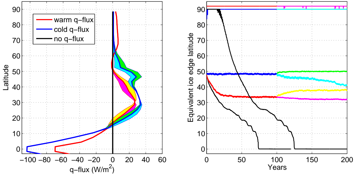
FIG. 10: Results from atmosphere-slab ocean runs with specified OHT. (left panel) Mean q-fluxes diagnosed from the Warm (red) and Cold (blue) states of Aqua. The green and yellow shadings indicate positively perturbed q-fluxes (i.e. poleward migration of the OHT convergence) while the cyan and magenta shadings indicate negatively perturbed q-fluxes (i.e. equatorward migration of the OHT convergence). (right panel) Time series of the equivalent sea ice latitude (see text) starting from the Warm (equivalent latitude of \sim 90^\circ ) and Cold (equivalent latitude of \sim 50^\circ ) states of the coupled GCM. The perturbed experiments are started from the equilibrated states of the unperturbed experiments and are displayed for years 100-200. The color coding of the curves corresponds to that used for the q-flux in the left panel.
