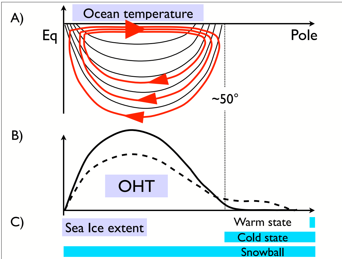
FIG. 9: Schematic of the multiple equilibrium states: A) ocean thermal structure (black) and residual overturning circulation (red), B) OHT transport in the Warm (dashed) and Cold (solid) states, and C) sea ice extent for the three stable states.
