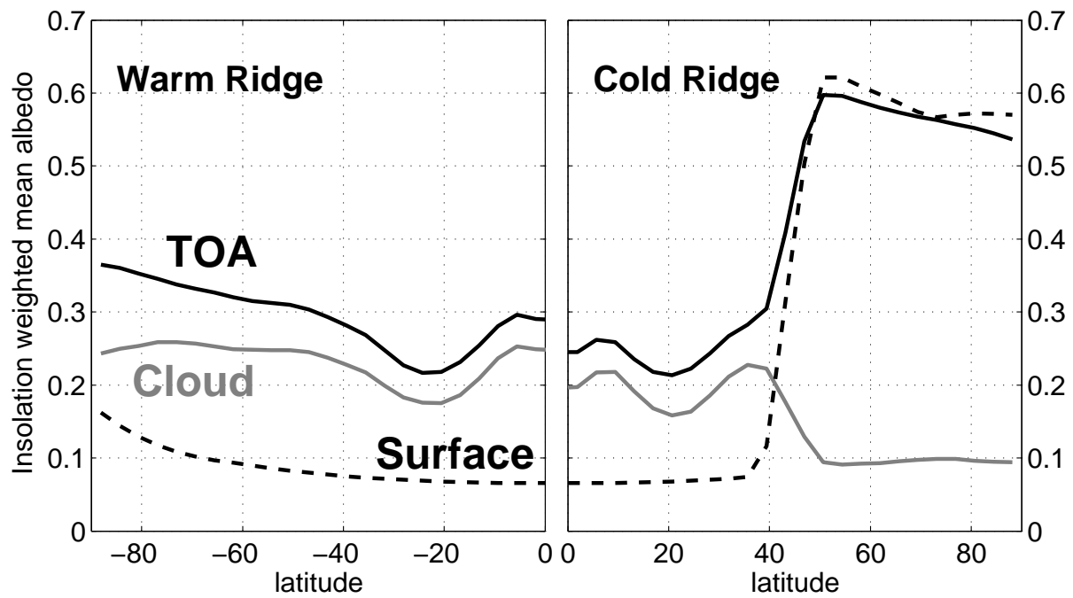
FIG. 7: Annual and zonal mean TOA (black), cloud (gray), and surface (dashed) albedos as a function of latitude for the Warm (left) and Cold (right) states of Ridge . See text for the details. Since the solutions are symmetric about the equator, only one hemisphere is plotted for each state. The Aqua results are very similar.
