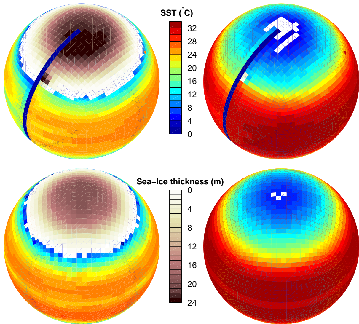
FIG. 1: SST and sea-ice thickness in Ridge (top) and Aqua (bottom) for the Cold (left) and Warm solutions (right).
