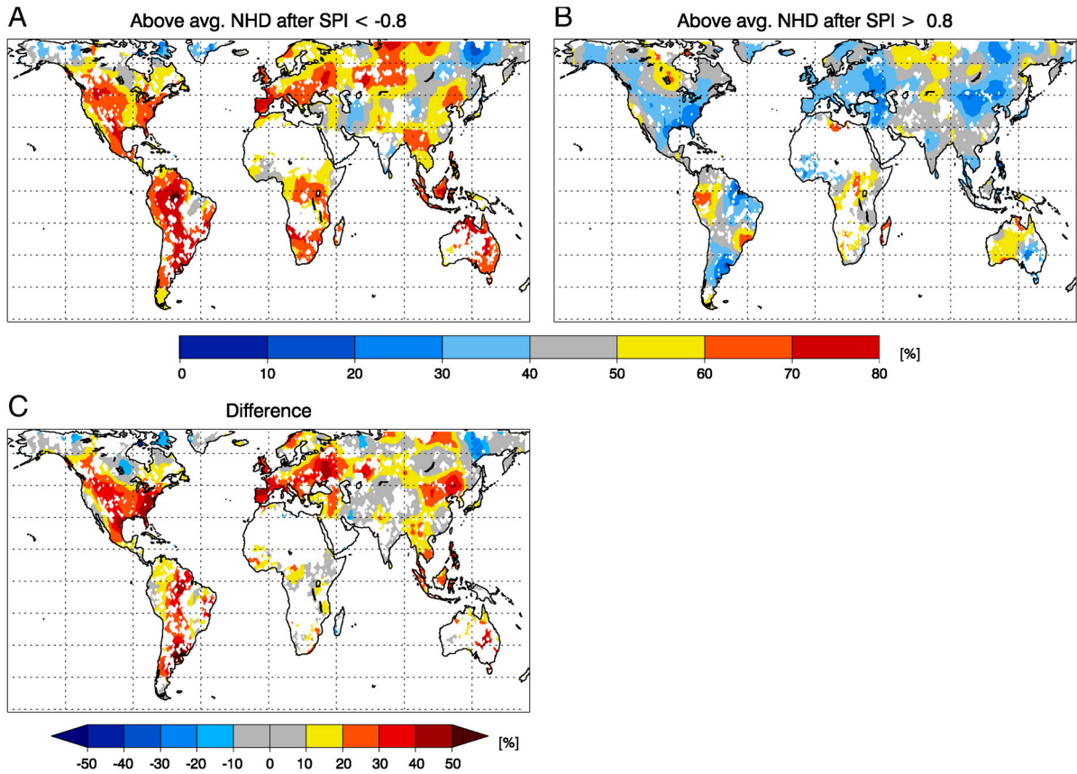
Fig. 4. Hot day occurrence probability after dry versus wet conditions. Occurrence probability for above-average number of hot days in the respective hottest month of each year following low 3-month SPI values (dry conditions, A ) and high 3-month SPI values (wet conditions, B ), and difference between the two ( C ). Values are given in percentage of years with above-average NHD from total number of low and high SPI years, respectively. Values that are based on a composite of less than 4 years are not shown (white areas). The employed datasets are ERA-Interim for NHD and CRU for SPI.
