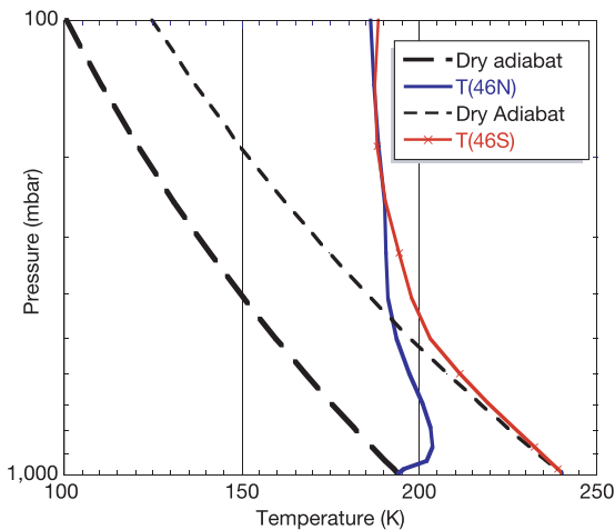
Figure 3 Typical January vertical temperature profiles for the 100 p.p.m. CO 2 case. For reference, the dry adiabat (virtually identical to the moist adiabat at these temperatures) is shown. Convection resets the temperature to the adiabat, so by comparing the actual curves with the adiabat, we can identify the layer in which convection causes the familiar sharp drop of temperature with height. T(46N) and T(46S) represent respectively the temperature profiles at latitudes 46° N and 46° S.
