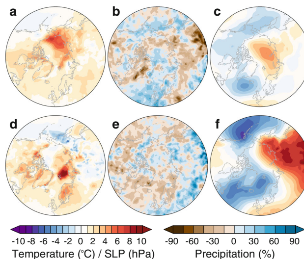
Fig. 9 Observed trends in autumn a near-surface temperature ( T_{ref} ), b precipitation ( P ) and c sea level pressure ( SLP ) for the period 1979–2009. Precipitation trends are expressed as percentages relative to the climatological-means. d–f As ( a–c ), but for winter. T_{ref} and SLP data are from the ERA-Interim reanalysis and P data are from the GPCP product
