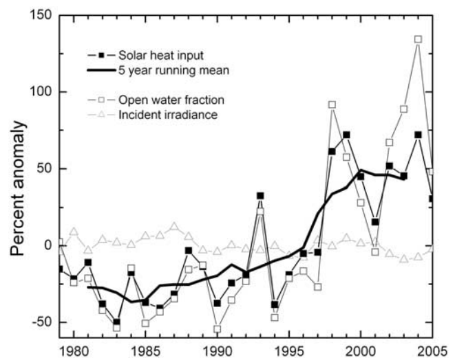
Figure 3. Time series of anomaly in annual solar heat input, open water fraction, and incident irradiance for a 75 \text{ km} \times 50 \text{ km} area centered on 76^\circ\text{N} , 170^\circ\text{W} . The thick line is the five year running mean of solar heat input.
