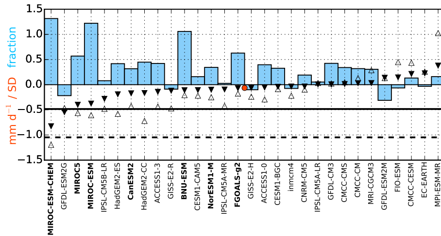
Figure 1. Past and future Sahel summer rainfall in CMIP5 coupled climate models. Blue bars show the change in central and eastern Sahel average summer rainfall (0–30° E, 10–20° N; July–September) by the end of the century (2071–2095) under RCP8.5 compared to the 1901–1999 average, as a fraction of that average. The seven models investigated in detail in this paper (Wet7 subset) are marked in bold. Filled triangles show the difference (drought minus non-drought) between the 1970–1989 drought period and the rest of the observational period (“non-drought”, 1901–1969 and 1990–2009), in \text{mm day}^{-1} . Open triangles show the same difference divided by the standard deviation of the non-drought period, in units of standard deviations. The solid and dashed horizontal lines show the respective observed values (CRU TS3.1; Harris et al., 2014). The orange circle indicates the median deviation from the observed drought–non-drought difference across the model ensemble; i.e., models shown to the left of this point are closer than average to the observed value.
