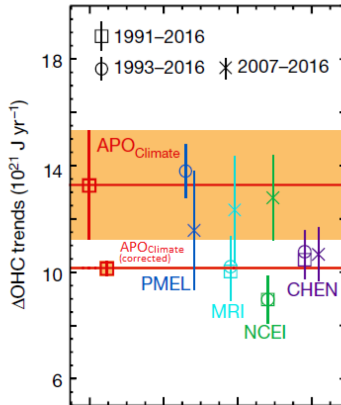
Figure 2. An adaptation of Figure 1b from Resplandy et al. with the corrected estimate for the \text{APO}_{\text{Climate}} derived \Delta\text{OHC} trend added (lower horizontal red line; no error bar is shown)
