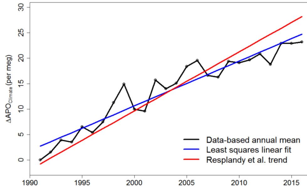
Figure 1. \Delta\text{APO}_{\text{Climate}} data values (black), the least squares linear fit (blue line) to them, and the linear trend per Resplandy et al. (red line)
