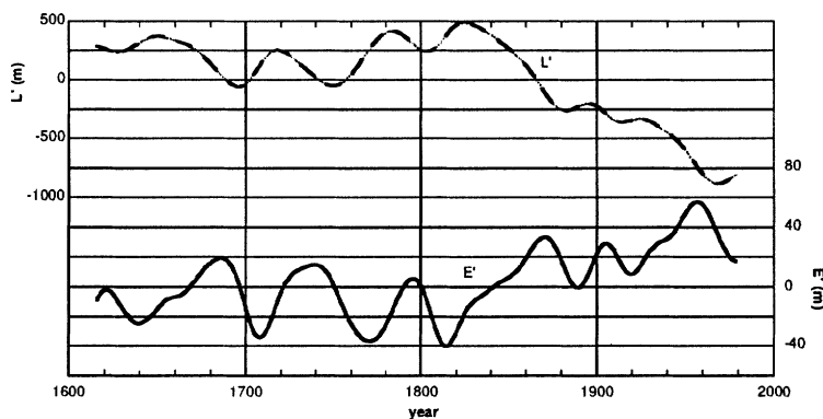
Figure 4 The length record of Glacier d'Argentière filtered with the Gaussian filter (dotted line) and the ELA reconstruction calculated with the analytical model (solid line).
