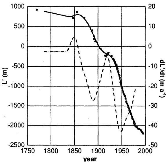
Figure 2 The length record of Hintereisferner filtered with the Gaussian filter and the time derivative of the length record (dashed line). The black dots indicate the individual data points.
