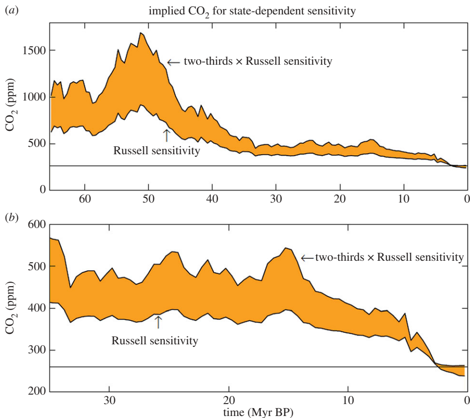
Figure 9. (a) \text{CO}_2 amount required to yield the global temperature history of figure 4a if fast-feedback climate sensitivity is that calculated with the Russell model, i.e. the sensitivity shown in figure 7b, and two-thirds of that sensitivity. These results assume that non- \text{CO}_2 GHGs provide 25% of the GHG climate forcing. (b) Vertical expansion for the past 35 Myr.
