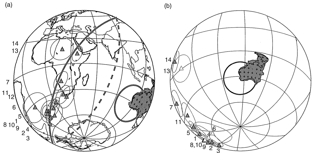
Figure 9 Example of a 'spinner diagram'. (a) Late Cryogenician–Ediacaran–Cambrian APW swath for Australia in the modern geographic reference frame. Fourteen critical poles, dated by biostratigraphy or relative stratigraphic position, appear widely dispersed, and the pole (with 95% confidence trace) to a great circle best-fitting thirteen of those poles lies near the western margin of the Australian Craton. (b) Rotation of Australia, its APW swath, and the swath's best-fitting great circle so that the pole to that swath lies at the center of an equal-area projection creating a 'spinner diagram'. If it is supposed that the back-and-forth time series comprising a continent's APW swath represents multiple (type II) TPW events at rates substantially faster than (or parallel to) plate motion; and if it is assumed, by reasoning outlined in the text and in Kirschvink et al. (1997) and Evans (1998, 2003) that the TPW axis lies on Earth's spin-equator, then because of geomagnetic polarity ambiguity in Neoproterozoic time, Australia's actual geographic location at most times during the interval spanning all proposed TPW events may be any rotationally equivalent location that preserves coincidence of its APW swath pole and the TPW axis. For the purposes of paleogeographic reconstruction, Australia's geomagnetic (= rotational) paleolatitude is constrained only for the discrete times of direct paleomagnetic constraints as represented by the individual poles. If rapid type II TPW oscillations were occurring on timescales of a few million years or less, then traditional comparisons of separate plates' paleolatitudes would be meaningless except in the rare instance of extremely precise agreement in pole ages from those plates. Each point on the Earth does, however, maintain a constant angular distance from a type II TPW axis, thus continents can be reconstructed relative to that reference frame. In practical terms from the figured example, Australia may be 'spun' around the (constantly equatorial) TPW axis shown in the center of the diagram. An alternative set of paleogeographic positions occupies the far hemisphere about the antipole to the TPW axis.
