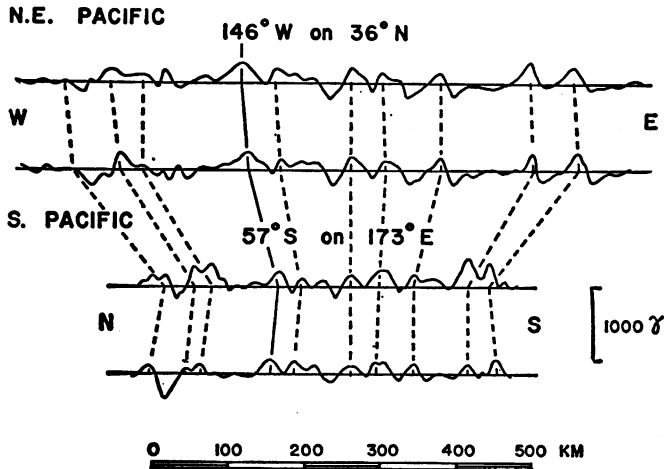
Fig. 16 (left). The anomaly pattern correlated between profiles by Peter and Raff in the North Pacific (37) and Christoffel and Ross in the South Pacific (38). It is suggested that the only difference between the two is the rate of spreading that formed them.
