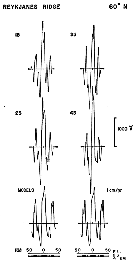
Fig. 5. Profiles observed across Reykjanes Ridge, together with computed profiles. The model to the left assumes the reversal time scale of Fig. 4; that to the right, the "revised" time scale of Figs. 12 and 13 (45). All observed and computed profiles have been drawn to the same proportion; 10 kilometers horizontally is equivalent to 100 gamma vertically (1 gamma = 10^{-5} oersted). F.L. , flight level.
