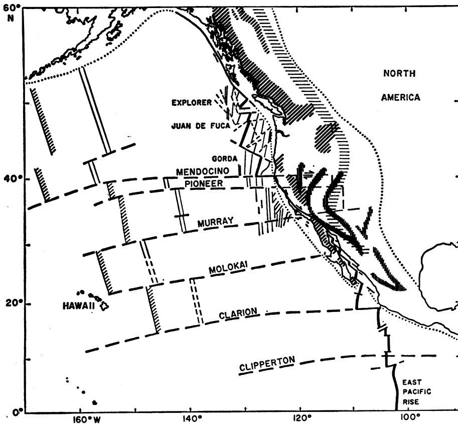
Fig. 15. The East Pacific Rise in the North Pacific. Solid black lines indicate the present crest and active transform faults [the crest south of the Gulf of California, from Menard (34)]. Thin lines represent key magnetic anomalies: in particular, the pair of anomalies traced by Peter (37) between 160° and 140°W. The half-herringbone pattern to the west suggests a possible boundary of the rise and its associated north-south magnetic anomalies. Broken lines indicate inactive faults or fractures. Dotted lines enclose the circum-Pacific cordillera within which the tectonic belts of Wise (28) are shown by ruled shading.
