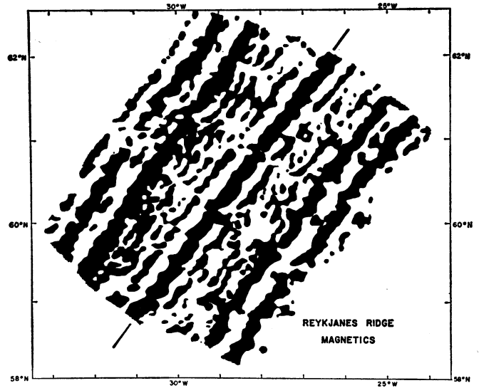
Fig. 2 (left). The location of Reykjanes Ridge, southwest of Iceland, and the area of Fig. 3. The 1000-fathom submarine contour is shown, together with the 500-fathom contours for Rockall Bank. Fig. 3 (right). Summary diagram of the magnetic anomalies observed over Reykjanes Ridge (see Fig. 2). Straight lines indicate the axis of the ridge and the central positive anomaly (17).
