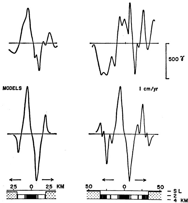
Fig. 10 (left). Observed profiles across the Red Sea [from Allan, Charnock, and Morelli (48); Drake and Girdler (26)] compared with computed profiles based on a constant rate of spreading and a truncated model and time scale according to the width of the central depression and zone of magnetic anomalies (49). Stippled area, "nonmagnetic" continental material. Fig. 11 (right). Inferred normal-reverse boundaries within the crust plotted against the reversal time scale of Fig. 4. The dashed line represents a similar plot for Juan de Fuca Ridge, if one assumes the earlier time scale—as did Vine and Wilson (8). Note the similar deviations from linearity for the East Pacific Rise and Juan de Fuca Ridge.
