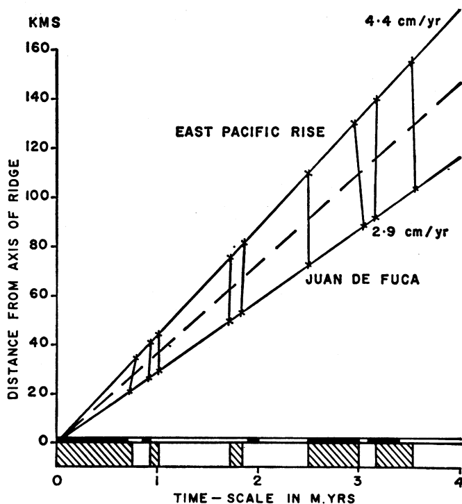
Fig. 12 (left). Crustal boundaries replotted along lines of constant rates of spreading (that is, best-fitting straight lines in Fig. 11); slight revision of the reversal time scale are suggested. The "revised" time scale is the lower, ruled scale. Fig. 13 (right). Magnetic boundaries across the East Pacific Rise, deduced out to 500 kilometers from the crest and plotted on a line representing a constant spreading rate of 4.4 centimeters per annum. Similar boundaries from Juan de Fuca Ridge are plotted out to 150 kilometers on the assumption of a constant spreading rate of 2.9 centimeters per annum. The time scale out to 5.5 million years is based on both plots. Beyond that time the time scale is based on the East Pacific Rise boundaries, and those deduced from Juan de Fuca Ridge are simply plotted on these time lines.
