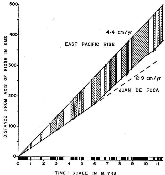
Fig. 12 (left). Crustal boundaries replotted along lines of constant rates of spreading (that is, best-fitting straight lines in Fig. 11); slight revision of the reversal time scale are suggested. The "revised" time scale is the lower, ruled scale. Fig. 13 (right). Magnetic boundaries across the East Pacific Rise, deduced out to 500 kilometers from the crest and plotted on a line representing a constant spreading rate of 4.4 centimeters per annum. Similar boundaries from Juan de Fuca Ridge are plotted out to 150 kilometers on the assumption of a constant spreading rate of 2.9 centimeters per annum. The time scale out to 5.5 million years is based on both plots. Beyond that time the time scale is based on the East Pacific Rise boundaries, and those deduced from Juan de Fuca Ridge are simply plotted on these time lines.
