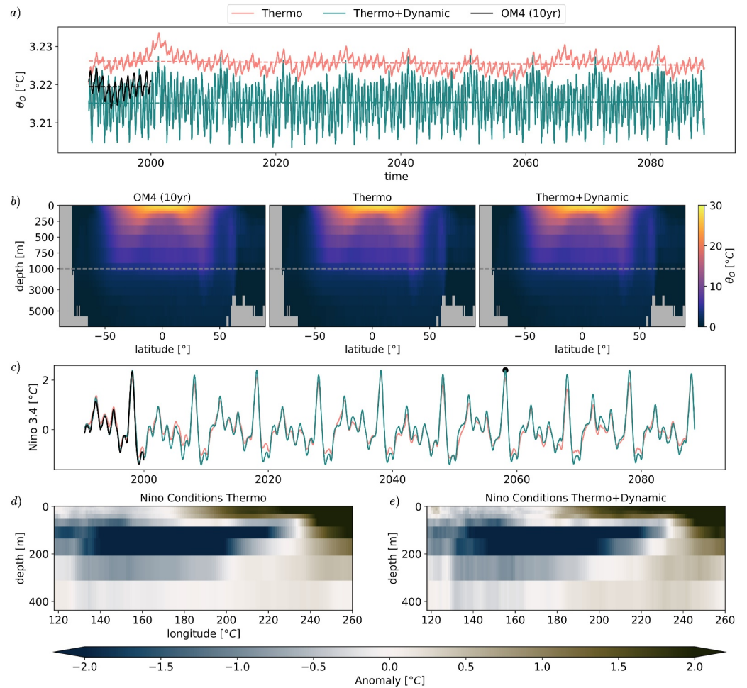
Figure 3. (a) Globally averaged potential temperature ( \theta_0 ) timeseries over a 100-year control run, comparing the 10-year ground truth OM4 (black) and predictions from F_{thermo} (red) and F_{thermo+dynamic} (green). (b) Time-averaged potential temperature ( \theta_0 ) depth profile over a 100-year control run, comparing the 10-year ground truth OM4 (left) and predictions from F_{thermo} (middle) and F_{thermo+dynamic} (right). (c) Nino 3.4 index timeseries over a 100-year control run, comparing the 10-year repeat for the ground truth (OM4, black) and predictions ( F_{thermo} , red; F_{thermo+dynamic} , green). (d)–(e) Meridionally averaged depth profile of potential temperature anomalies in the tropics during the peak Nino event (marked by a black dot in the timeseries) over the test set for F_{thermo} (d) and F_{thermo+dynamic} (e). Anomalies are as in Figure 2.
