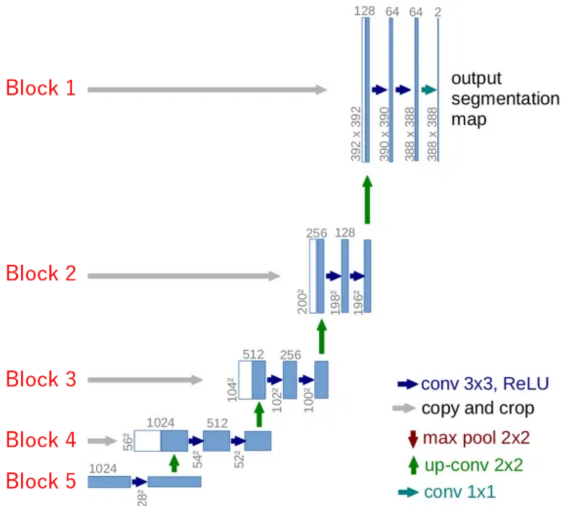
The expanding path of the U-Net.
