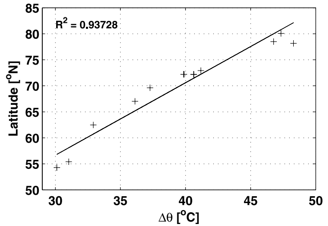
Figure 7. Extent of switch-like sea ice growth (vertical axis, in degrees) versus the initial atmospheric temperature gradient in °C (horizontal axis). The extent of switch-like sea ice growth is defined to be the southernmost latitude with sea ice immediately after the switch-like sea ice expansion. Each plus sign marks an experiment with different initial meridional temperature gradient (including those that appear in Table 6), while the solid line is a linear fit. The sea ice extent plotted here is calculated, for all model runs, 1000 years after the continental ice sheet had reached its threshold value and sea ice started growing.
