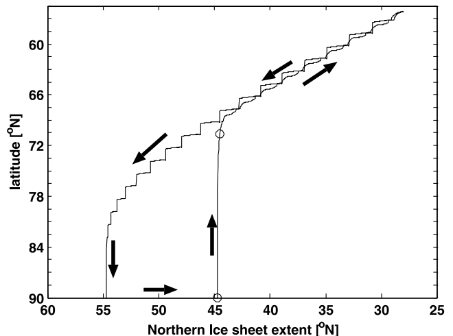
Figure 8. Hysteresis between the land ice extent (horizontal axis) and sea ice extent (vertical axis). Extent of both sea ice and land ice is defined as the southernmost latitude with sea or land ice, respectively. This plot was obtained by slowly increasing and then decreasing the land ice volume using the 1.5° resolution version of the coupled model. Circles denote beginning and end of sea ice growth, as in Figure 5.
