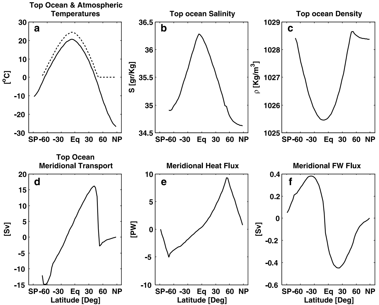
Figure 3. Model solution for typical glacial-like boundary conditions of northern ice sheet extending to 55^{\circ}\text{N} . Shown as a function of latitude are (a) atmospheric temperature (solid line) and ocean top layer temperature (dashed line) in ^{\circ}\text{C} , (b) upper ocean salinity (parts per thousand), (c) density of the upper ocean layer ( \text{kg m}^{-3} ), (d) meridional transport in upper ocean (sverdrup (Sv)), (e) atmospheric meridional heat flux (PW), and (f) meridional atmospheric freshwater (FW) flux (Sv).
