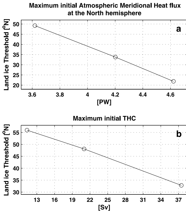
Figure 6. The critical northern ice sheet extent at which sea ice starts to grow (the latitude of the southern edge of the continental ice sheet, in degrees) as a function of the (a) maximum (over all latitudes) initial steady state atmospheric meridional heat (PW) for runs C_1 – C_3 in Table 6 and (b) maximum (over all latitudes) of the initial steady state meridional thermohaline circulation (THC) (Sv), runs r_{o1} – r_{o3} in Table 6.
