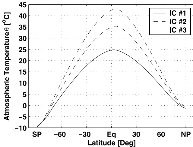
Figure 4. Three profiles of steady state atmospheric temperature ( ^{\circ}\text{C} ). These profiles were used as initial conditions (IC) for the model experiments examining the response of the sea ice to a slow equatorward expansion of the continental ice sheet. Each of the three steady states, denoted by IC 1 (solid line), IC 2 (dashed line), and IC 3 (dash-dotted line), was obtained for a particular set of model parameters, given in Table 5.
