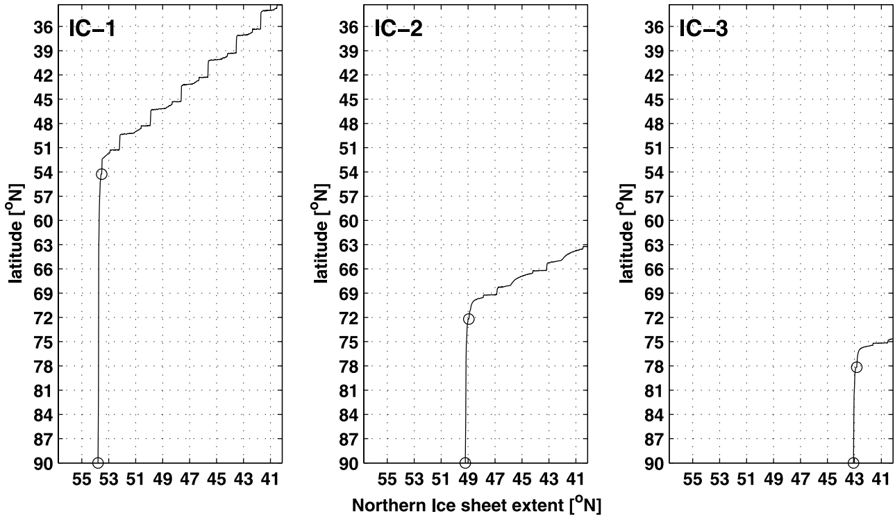
Figure 5. Results for the model runs with specified constant rate of ice sheet growth over a period of 100 kyr, starting with the three different initial conditions IC 1, IC 2, and IC 3 shown in Figure 4. Shown is the sea ice extent (southernmost ocean cell with sea ice) as a function of the land ice extent (the southernmost latitude to which the Northern Hemisphere ice sheet extends). The straight vertical segment in these plots corresponds to the rapid, switch-like sea ice growth. After the rapid growth, sea ice continues to expand slowly with the growing land ice. The two circles in each plot mark the beginning of the sea ice growth and 1000 years later. Therefore these two circles mark the time interval in which sea ice grows in a switch-like manner.
