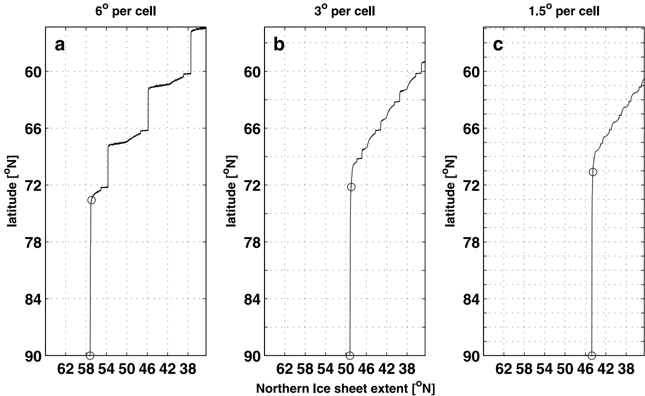
Figure 9. Plots of the sensitivity to model resolution. Shown is the sea ice extent as a function of slowly increasing land ice sheets for model runs with meridional resolutions of (a) 6^\circ , (b) 3^\circ , and (c) 1.5^\circ per cell. Besides the atmospheric time step that is halved in the higher-resolution experiments to keep the model stable, all other model parameters and initial conditions are the same for all three runs. The horizontal axis shows the latitude of the southernmost edge of the northern ice sheet. The vertical axis shows the southernmost latitude with sea ice in the Northern Hemisphere. The circles indicate the beginning of the sea ice growth and a time mark of 1000 years later. The switch-like sea ice growth and its meridional extent (the distance between the two circles) are clearly very similar for all three resolutions. The threshold value of the continental ice sheet extent which triggers sea ice growth does seem sensitive to the meridional resolution.
