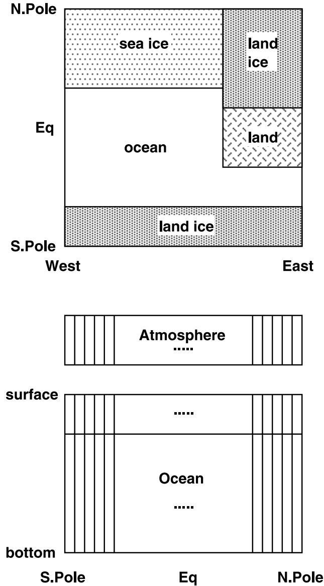
Figure 2. Model geometry. (top) Top view (latitude versus longitude) of the land, land ice, ocean, and sea ice distributions. (bottom) Latitude versus depth cross section through the ocean and atmosphere models. The vertical lines schematically mark a few of the grid boxes in the atmosphere and ocean. The latitudinal resolution (the latitudinal extent of these grid boxes) varies in the runs presented here from 6^\circ to 1.5^\circ .
