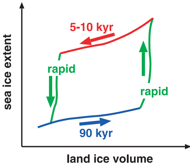
Figure 1. A schematic figure of the hysteresis between land ice and sea ice during glacial cycles, predicted using a simple box model by Gildor and Tziperman [2000] and examined here using a model that is continuous in the meridional direction.
