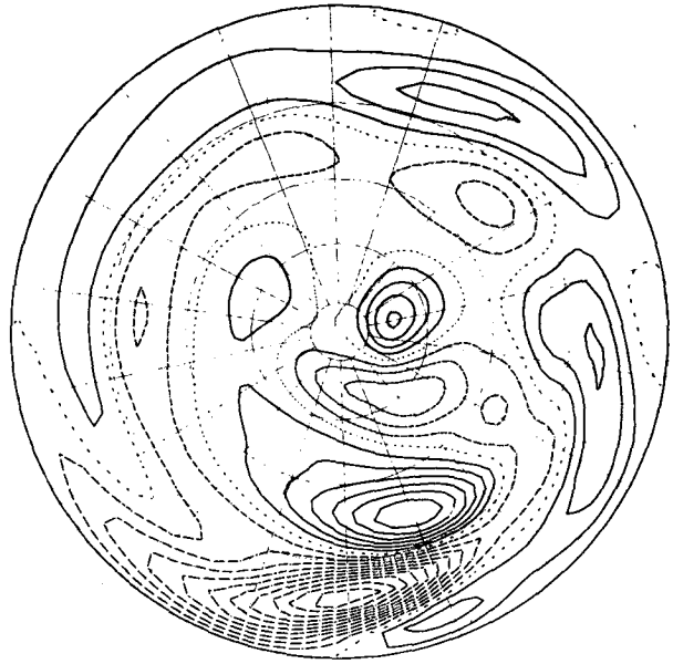
FIG. 1. 30-day average perturbation vorticity field for a negative vorticity source in the region 0–30°N, 30°W–30°E switched on at t = 0 using a hemispheric barotropic model linearized about a Northern Hemisphere 300 mb winter zonal flow. The map projection is polar stereographic with lines of latitude and longitude drawn every 20°. Negative contours are dashed, the zero contour dotted and positive contours continuous. With magnitudes specified in the text, the contour interval is 0.05Ω.
