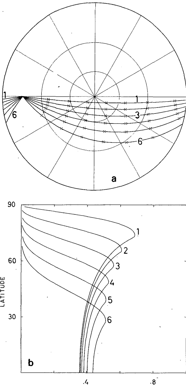
FIG. 12. (a) Rays and phases marked by a cross every 180° for a source at 15° in a super-rotation flow. If all wavelengths give a negative extremum at the source, the crosses mark the positions of successive positive and negative extrema. Lines of latitude and longitude are drawn every 30° and the zonal wavenumbers associated with the rays are indicated. (b) Amplitudes of the extrema on the rays for the different zonal wavenumbers, on the super-rotation flow shown as a function of latitude. The relative amplitudes of the different wavenumbers depend on the position and nature of the source.
