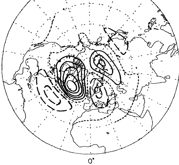
FIG. 11. The western Atlantic pattern at 500 mb found by Wallace and Gutzler (1980, adapted from their Fig. 21). Shown is the difference between the 10 months with the largest positive value of an index of the pattern and the 10 months with the largest negative values in a set of 45 winter months. The contour interval is 4 dam. Interpreting the contours as in Fig. 3, the picture may be taken as typical of the winter months with a large positive value of the index.
