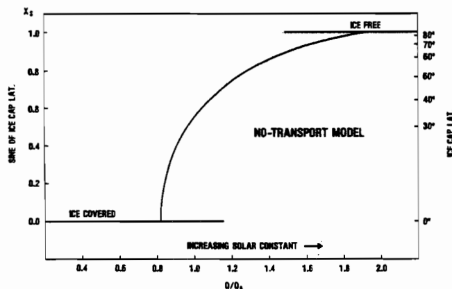
Fig. 3. Sine of steady state ice cap edge latitude x_i versus solar constant in units of its present value for a one-dimensional climate model with no horizontal heat transports (cf. equation (17)).
