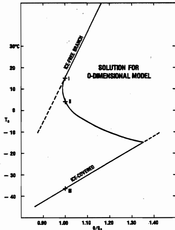
Fig. 2. Steady-state temperatures corresponding to the climate solutions for the zero-dimensional climate model with variable ice cap as a function of solar constant in units of its present value (solid curve). The roots I, II, and III correspond to those in Figure 1. The dashed curves show the solutions that would be obtained in the case of infinite horizontal heat transport in which the planet is isothermal.
