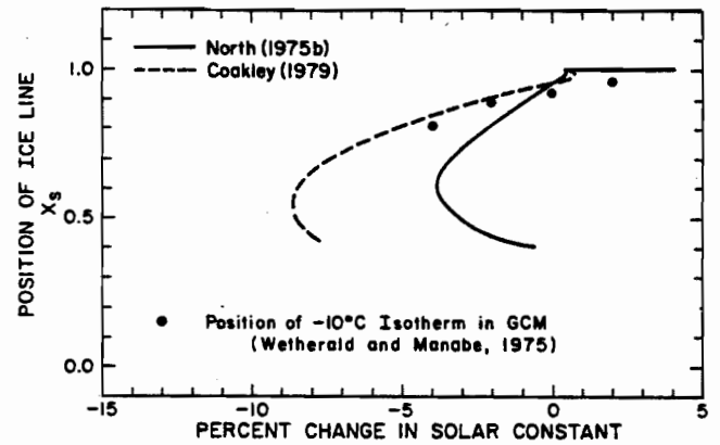
Fig. 14. Equilibrium position of the ice line ( -10^\circ\text{C} isotherm) as a function of the solar constant. Results obtained with radiation parameterizations adopted by North [1975b] (solid curve) and by Coakley [1979] (dashed curve). For comparison the positions of the -10^\circ\text{C} isotherm of the lowest GCM level from calculations performed by Wetherald and Manabe [1975] are represented by circles [Coakley, 1979].
