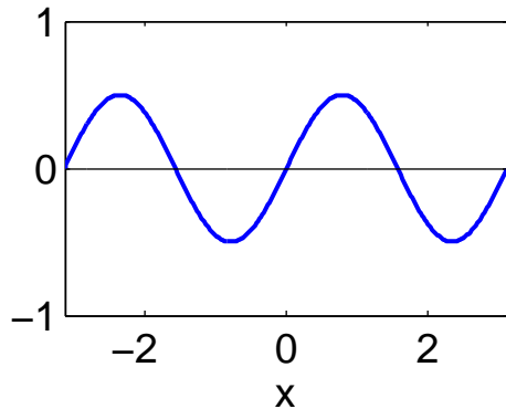
\cos(1\pi x/L) \times \sin(1\pi x/L)
