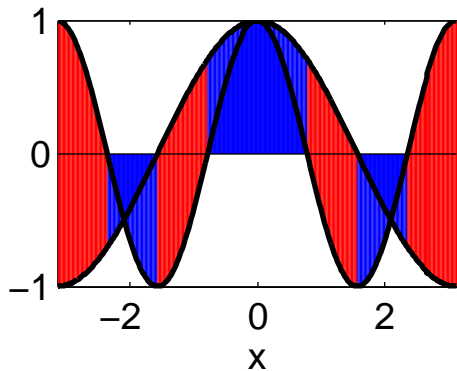
\cos(1\pi x/L) \times \cos(2\pi x/L)
